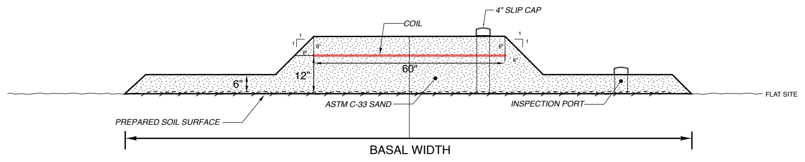
Section A NTS
