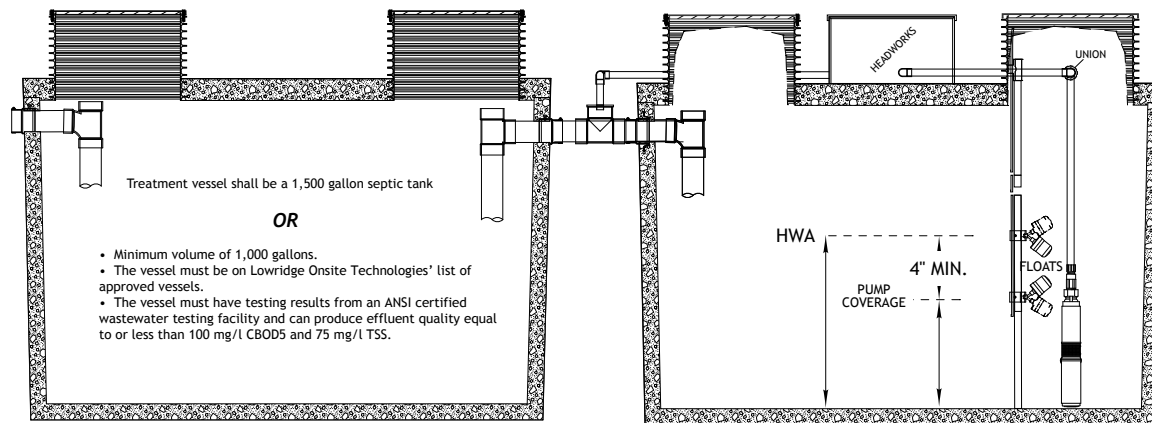
CROSS SECTION
