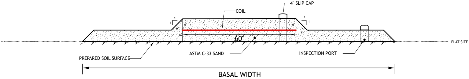
Section A NTS
