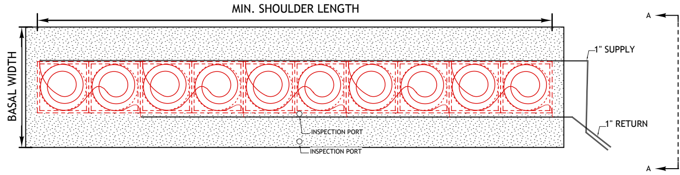
Plan View NTS
