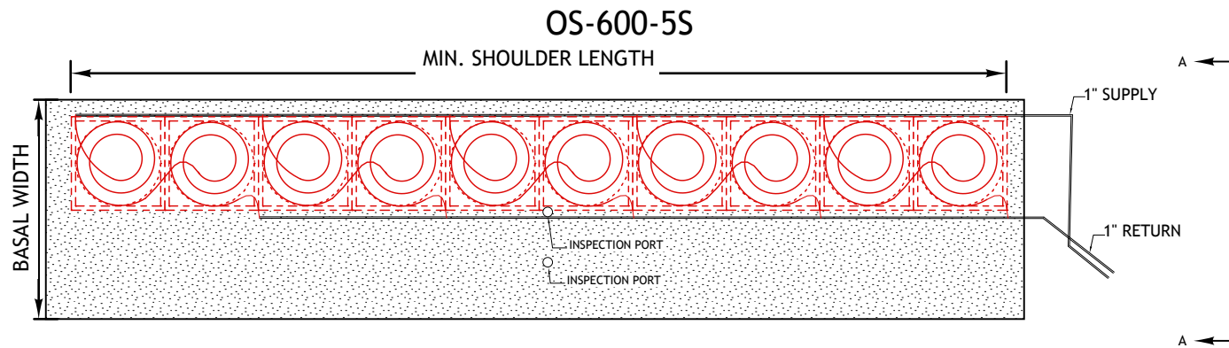
Plan View NTS
