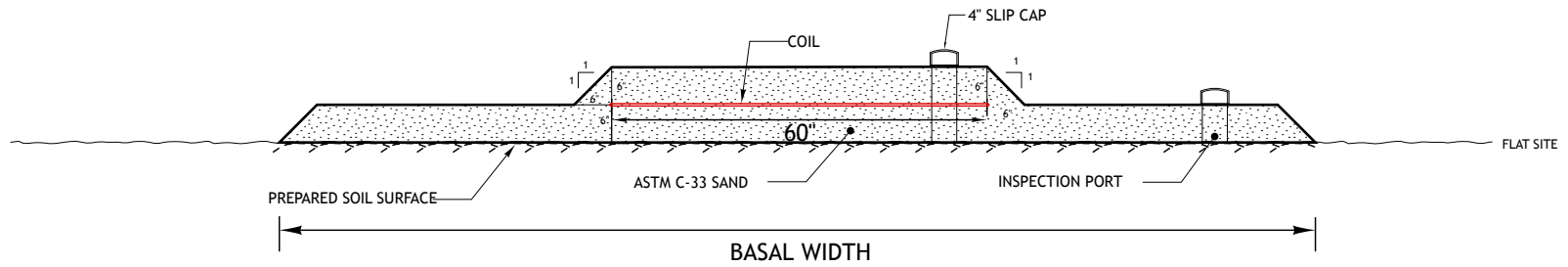
Section A NTS
